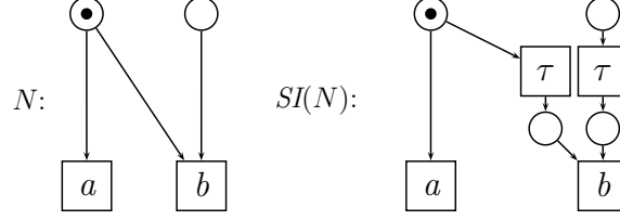
Fig. 3. The transition a can be refused in SI(N) by firing the left \tau .
